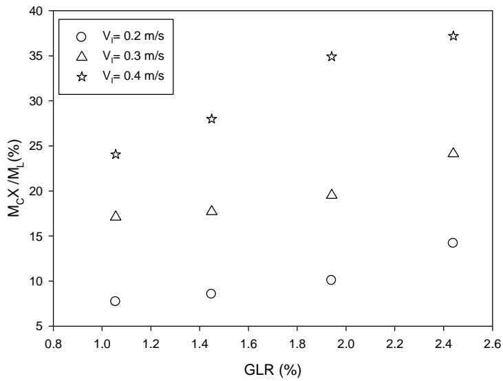
Figure 4: Percentage of total injected liquid which is free liquid after injection versus GLR for 3 different fluidization velocities during injection
